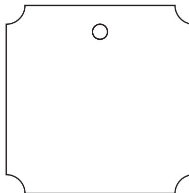
C23 50x50mm 4mm hole
